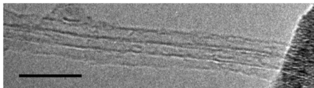
FIGURE 4. A TEM image of the PPEI-EI-SWNT sample on a holey LaCrO 3 stainless steel grid after thermal defunctionalization at 370 °C with air (scale bar = 10 nm). 23
