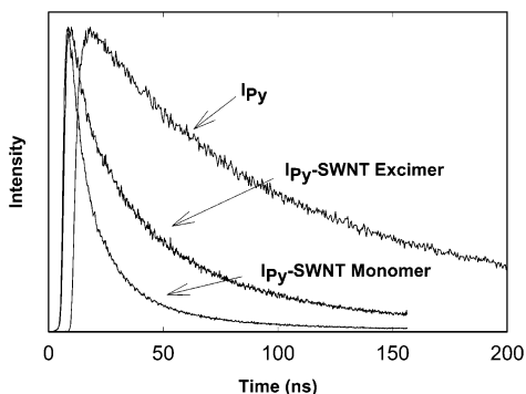
FIGURE 12. Fluorescence decays of I_{\text{Py}} and I_{\text{Py-SWNT}} (monitored at 380 nm for monomer and 490 nm for excimer) in room-temperature toluene. Reprinted with permission from ref 43. Copyright 2002 American Institute of Physics.
