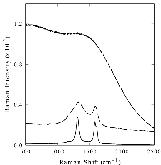
FIGURE 10. Raman spectra (780 nm excitation) of the I-MWNT sample before (—) and after (—•—) thermal defunctionalization in a TGA scan to 650 °C. The spectrum of the pristine MWNT sample (—) is also shown for comparison. 36
